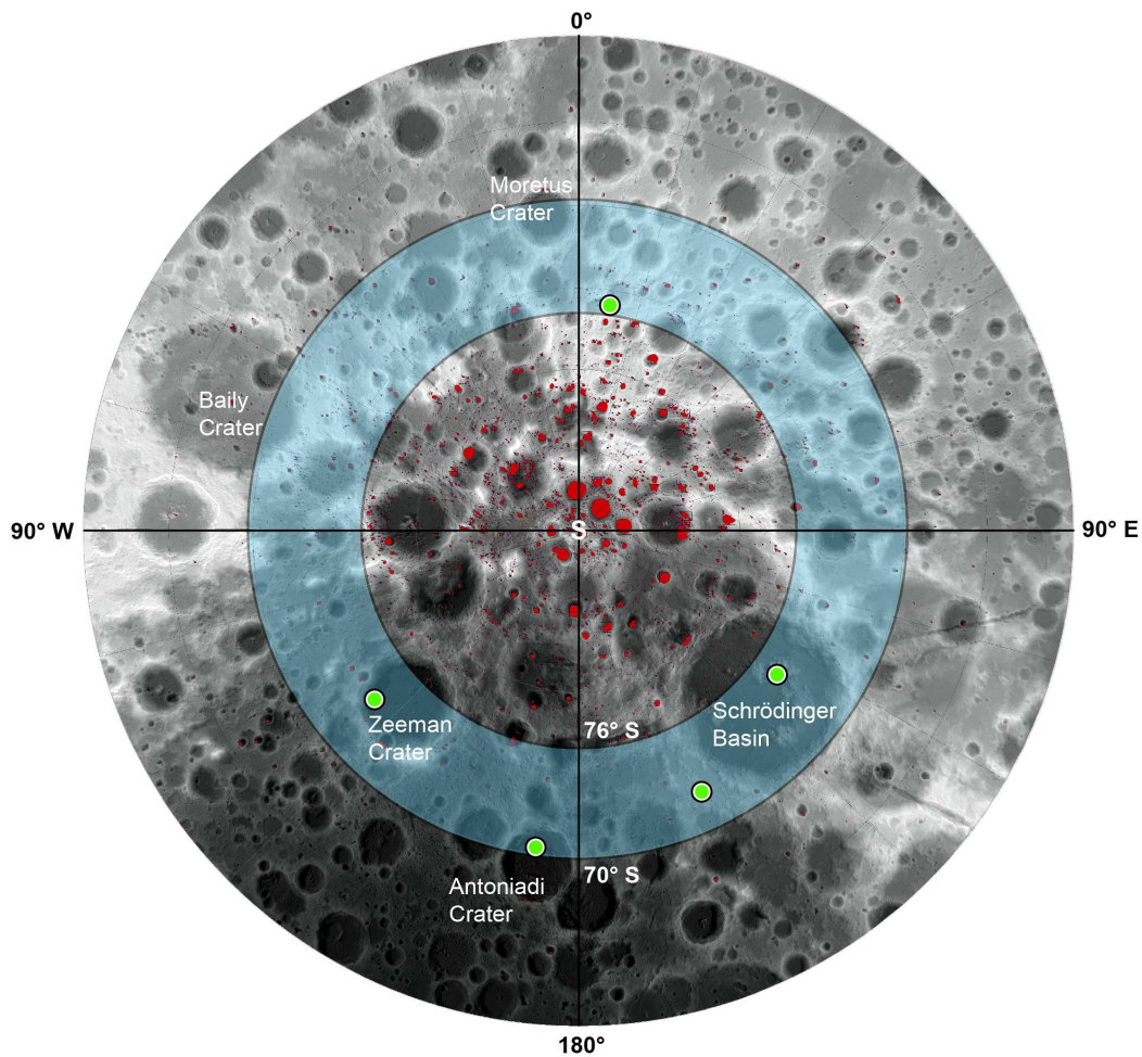
Figure A.2: A south polar view of the Moon with permanently shadowed regions (PSRs) highlighted in red (per McGovern et al. (2013) ) and the location of identified PSR boulder tracks in green. The blue band area represents the region where boulder tracks were observed in PSRs, located between \sim 70^\circ and 76^\circ latitude, that is, the region where secondary illumination and image processing still allow to use NAC images without compromising spatial resolution.
