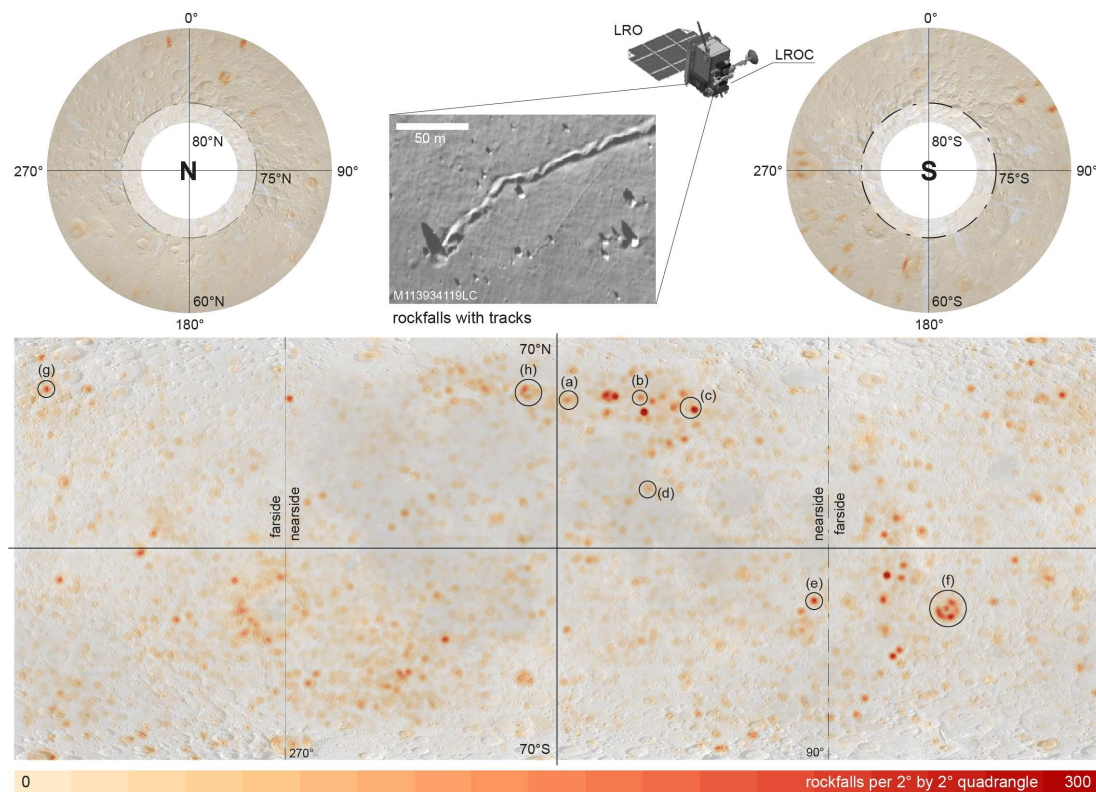
Figure 3.1: Global rockfall distribution heat map. Heat maps of lunar global rockfall distribution in both equiarectangular ( 70^{\circ} N to 70^{\circ} S) and polar projection ( 60^{\circ} N to 80^{\circ} N and 60^{\circ} S to 80^{\circ} S). Mapping results above 75^{\circ} N and below 75^{\circ} S might be less complete due to challenging illumination conditions (indicated by transparent white areas). Rockfall density is given in rockfalls per square degrees, i.e., the number of rockfalls per 2^{\circ} longitude quadrangle. The labeled black circles denote details shown in Figure 3.2. Inset shows examples of rockfalls and their tracks with various sizes: detail of LRO NAC (LROC) image M113934119LC. Global WAC mosaic in the background (Wagner et al., 2015). NAC image credits to LROC/ASU/NASA.
