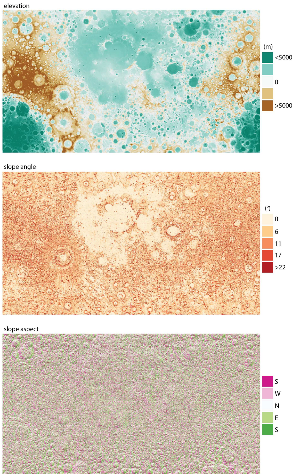
Figure A.36: Auxiliary maps (elevation, slope angle, slope aspect) as used for this study (Mercator projections, 70°N to 70°S, 180°W to 180°E, for visualization only). Please refer to the references cited in section 3.2 (main paper) and Table A.7 for more details.
