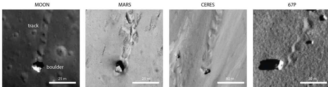
Figure 2.13: Examples of rockfalls (boulder and track) from the Moon (NAC), Mars (HiRISE), Ceres (FC), and comet 67P (OSIRIS) showcasing similarities and differences in physical appearance; details of M138107059LC, ESP_039901_1665, FC11B0005064_18168115057F1G, and N20160605T150621617ID30F22.
