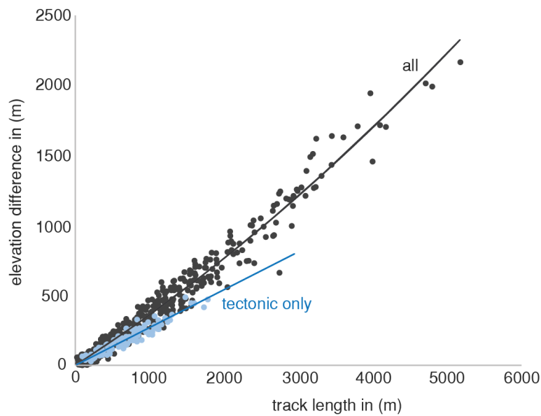
Figure A.48: Relation between track length and elevation drop for the cumulative (black, non-linear) and tectonic (blue, quasi-linear) rockfall populations as measured in the thirteen studied Aols.
