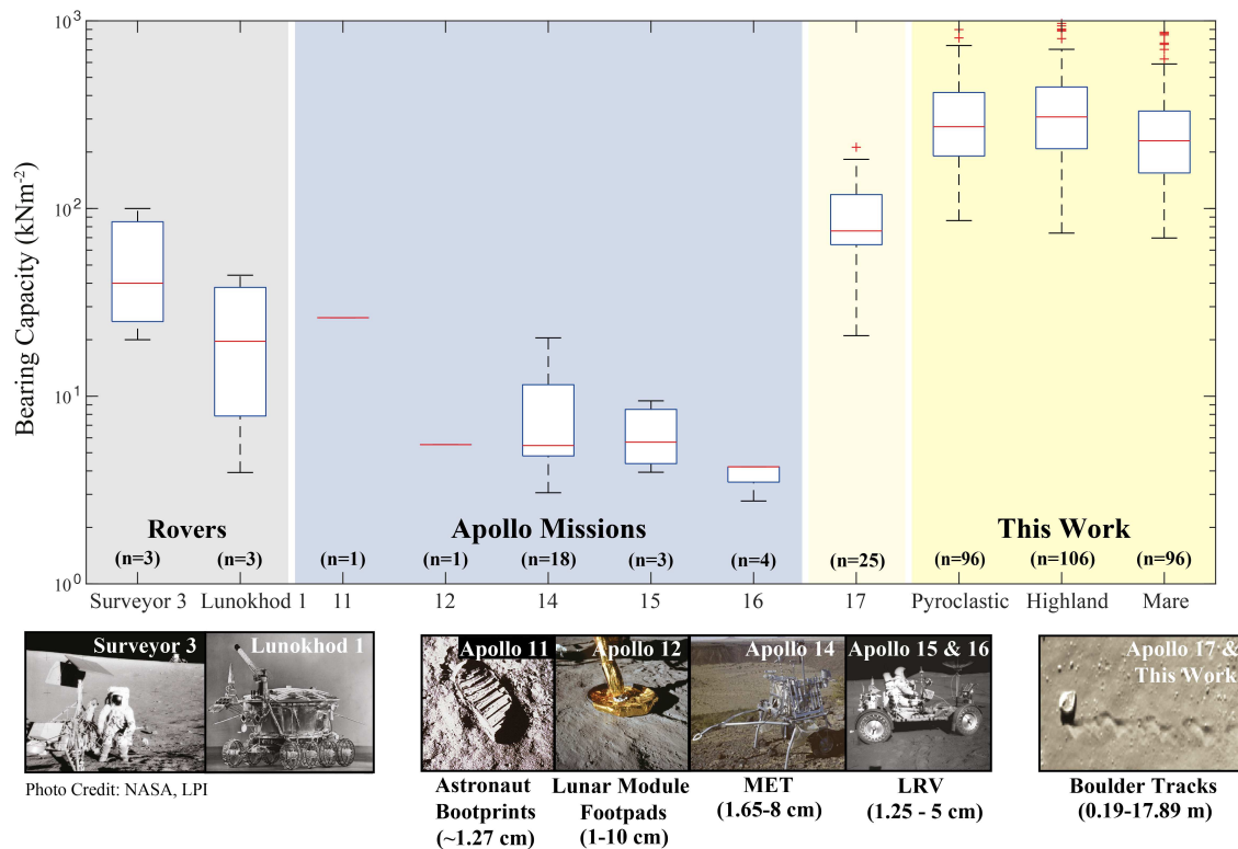
Figure 4.4: Comparison of bearing capacity values in this work and those calculated from literature values, including from different vehicles and objects, that is, astronaut bootprints, rover wheels, lander footpads, and rockfalls (Jaffe, 1971). Values used in calculations are taken from Apollo preliminary science reports 11-17 (Mitchell et al., 1972a, 1973, 1974). Lunokhod 1 bearing capacity values have not been calculated with the method presented in this paper but have been transferred from kg/cm 2 to kN/m 2 (Basilevsky et al., 2015). Bearing capacity values are dependent on depth; that is, small bearing capacity values reflect shallow penetration depths of the respective vehicle (e.g., landing pads). Black lines in box plots indicate the median of the respective data set, and red crosses indicate outliers. Highland and mare data are taken from widespread locations, and the average regolith thicknesses within those materials, from the literature, are used to constrain estimated regolith thickness. This explains overlap in sample numbers.
