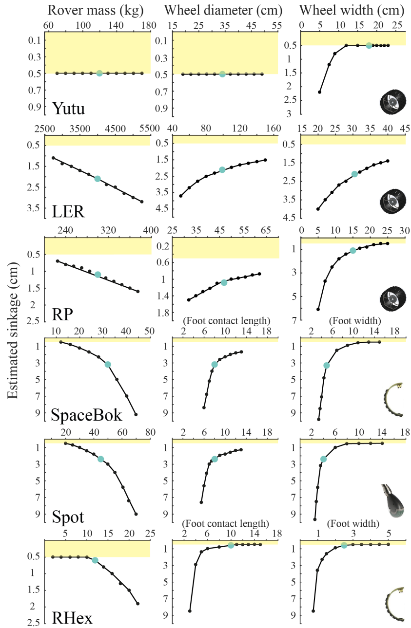
Figure 4.5: Yutu, LER, RP, SpaceBok, Spot, RHex type rover estimated sinkage as function of difference in mass, wheel diameter/foot contact length, and wheel/foot width, based on derived bearing capacity values. All wheels/legs touch the ground. Cyan point denotes the sinkage using the default vehicle design specifications. Shaded area marks depth range from 0 to 0.5 cm, where sinkage has not been calculated. Vehicle specifications have been taken or inferred from Carrier et al. (1991), Asnani et al. (2009), ESA (n.d.a), ESA (n.d.b), W. J. Bluethmann (pers. comm., 2018), NASA (2010), Boston-Dynamics (2019), SpaceBok (2017), and photographs/blueprints (where information was not directly accessible). Vehicle details are available in Table A.9. SEV = Space Exploration Vehicle; RP = Resource Prospector; LER = Lunar Electric Rover.
