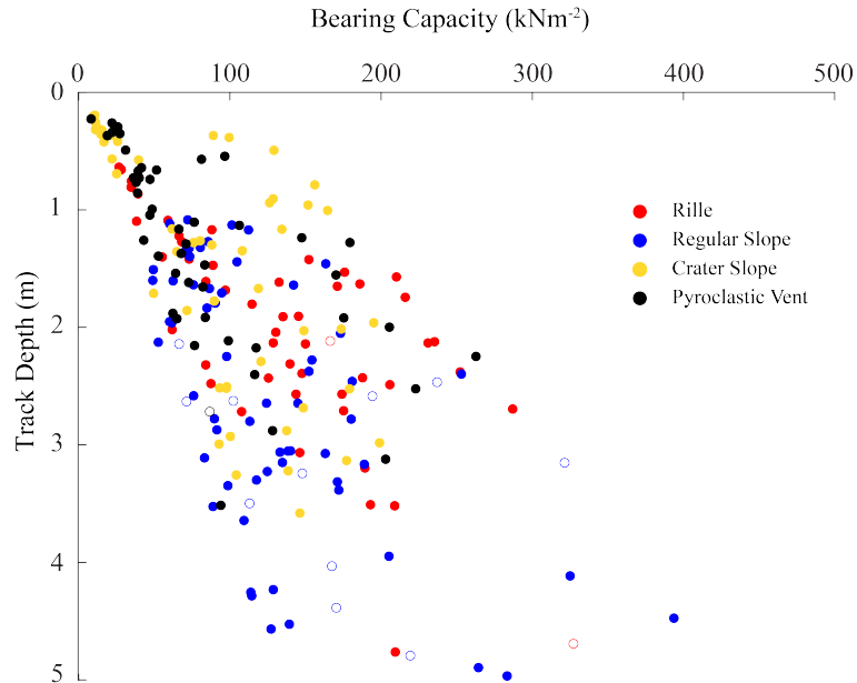
Figure A.60: The bearing capacity values for each boulder site in geomorphological context are presented as a function of track depth. Hollow shapes indicate boulders that are believed to have cut through the regolith at their location based on estimated taken from sources listed in Table A.12/ Figure A.56.
