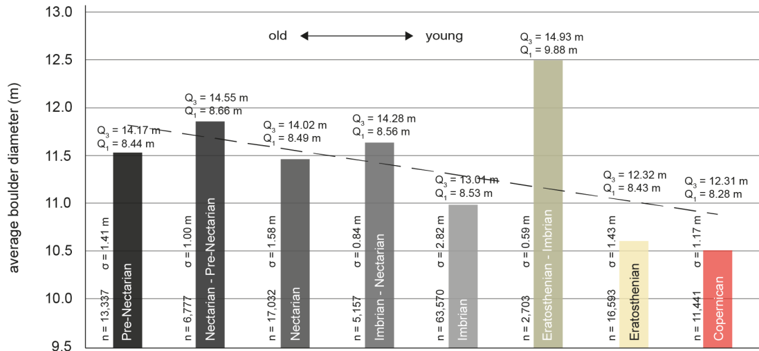
Figure A.30: Average boulder diameter as function of terrane age. Rockfalls in older terranes show systematically larger average boulder diameters, as highlighted by the linear fit. The used number of rockfalls ( n ), the standard deviation ( \sigma ), and the first and third quartiles ( Q_1 and Q_3 ) of each age class are shown.
