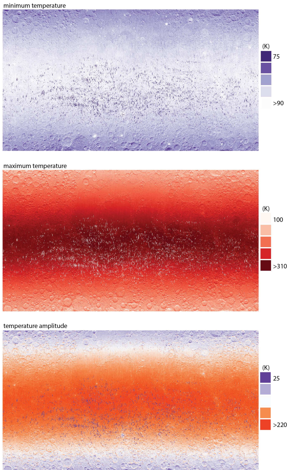
Figure A.38: Auxiliary maps (minimum temperature, maximum temperature, temperature amplitude) as used for this study (Mercator projections, 70°N to 70°S, 180°W to 180°E, for visualization only). Please refer to the references cited in section 3.2 (main paper) and Table A.7 for more details.
