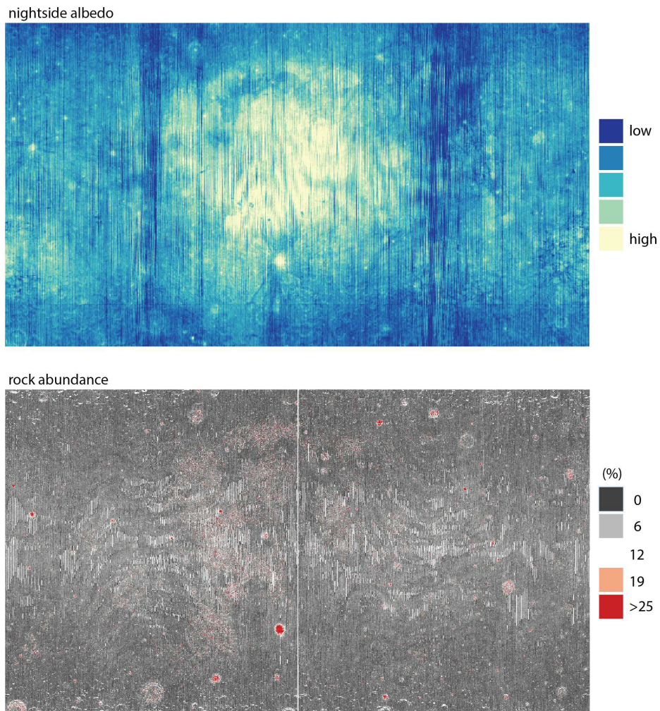
Figure A.40: Auxiliary maps (nightside albedo, rock abundance) as used for this study (Mercator projections, 70°N to 70°S, 180°W to 180°E, for visualization only). Please refer to the references cited in section 3.2 (main paper) and Table A.7 for more details.
