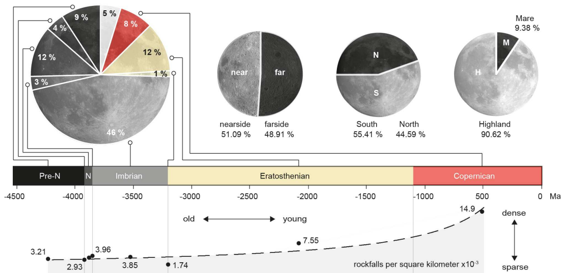
Figure 3.3: Statistics about rockfall distribution in space and time. Statistics highlight the spatial distribution of rockfalls and its implications. More rockfalls occur in highland terranes and the majority of rockfalls occur in Imbrian terranes, while Nectarian (N) and even pre-Nectarian sites (pre-N) feature a substantial number of recent rockfalls ( \sim 25\% ). Owing to inaccuracies in the underlying geologic map, the number of rockfalls in ancient terranes is potentially reduced in favor of the Copernican and Eratosthenian bins (see Supplementary Figure A.34). The normalization of the CNN-derived rockfall counts over area in the regions provides a first-order estimate (power law fit, black dashed line) of the advective erosion rate of the lunar topography and its evolution over time (Equation 3.1 in the "Methods" section). Geologic lunar timescale based on Hawke et al. (2004) and Neukum et al. (2001) .
