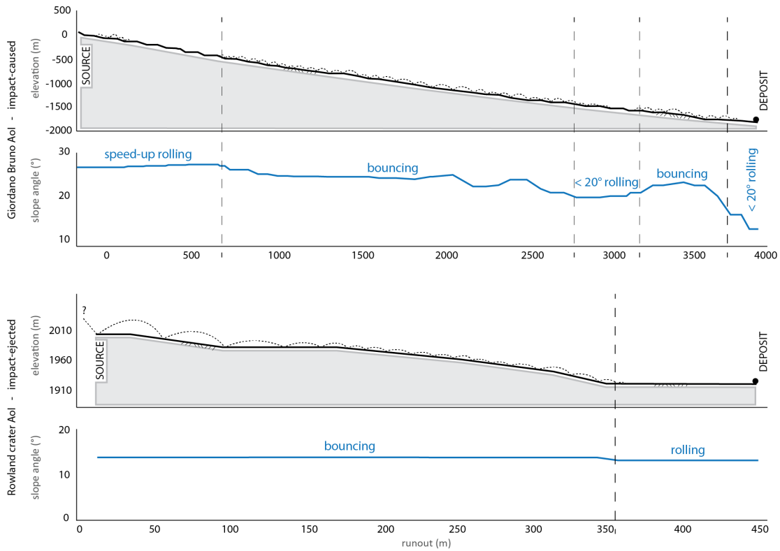
Figure A.47: Example rockfall trajectories from the Giordano Bruno (impact-caused) and Rowland crater (impact-ejected) Aols. Top: topographic cross-section, bottom: slope angle along the trajectory. The dashed black line represents the trajectory of the rockfall. Bounce widths represent real observations, bounce heights are reconstructed. The x and y axes are not to scale.
